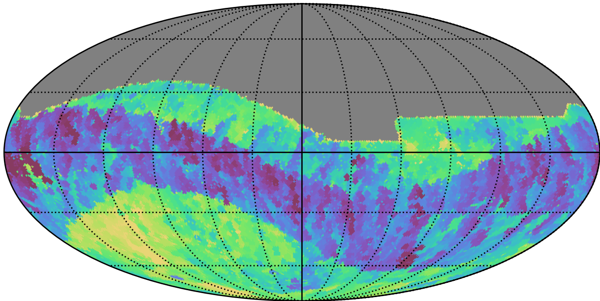
no_high_blob_v3.3_10yrs All sky z band: Min fiveSigmaDepth
