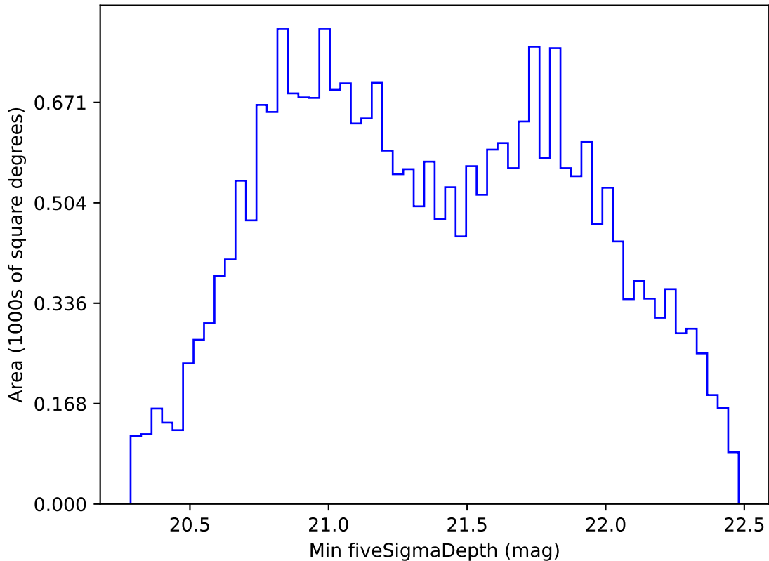
no_high_blob_v3.3_10yrs All sky z band: Min fiveSigmaDepth
