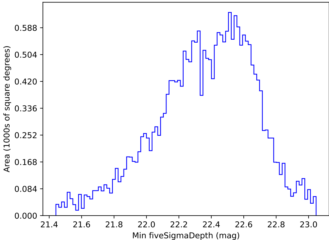
no_high_blob_v3.3_10yrs All sky u band: Min fiveSigmaDepth
