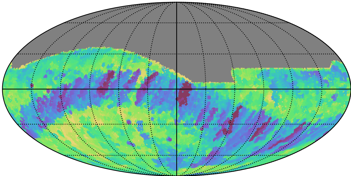
no_high_blob_v3.3_10yrs All sky r band: Min fiveSigmaDepth
