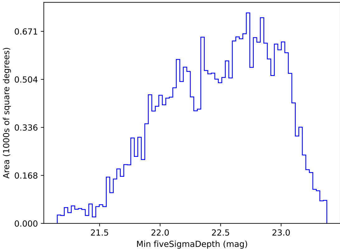
no_high_blob_v3.3_10yrs All sky r band: Min fiveSigmaDepth
