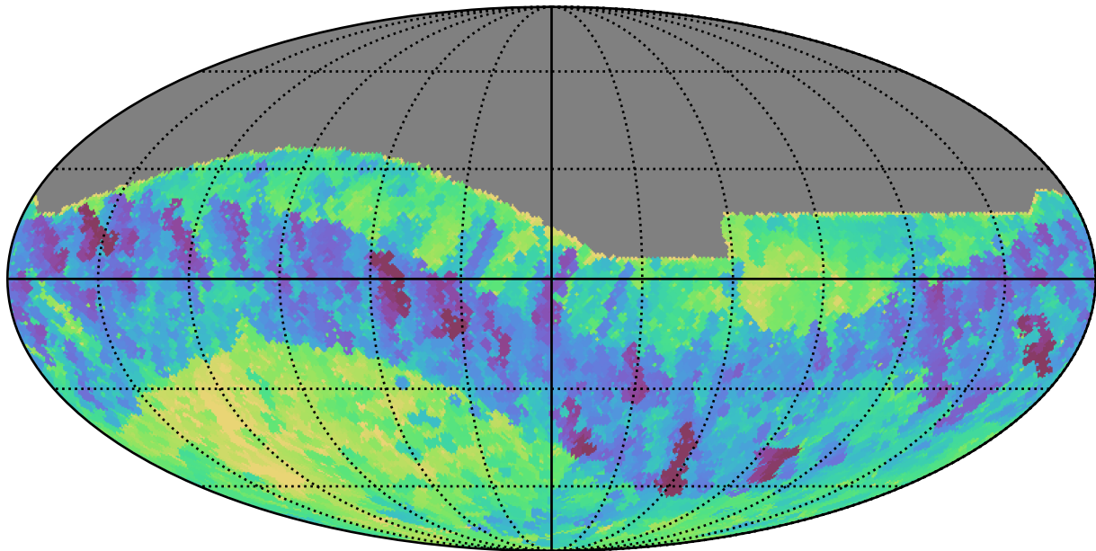
no_high_blob_v3.3_10yrs All sky i band: Min fiveSigmaDepth
