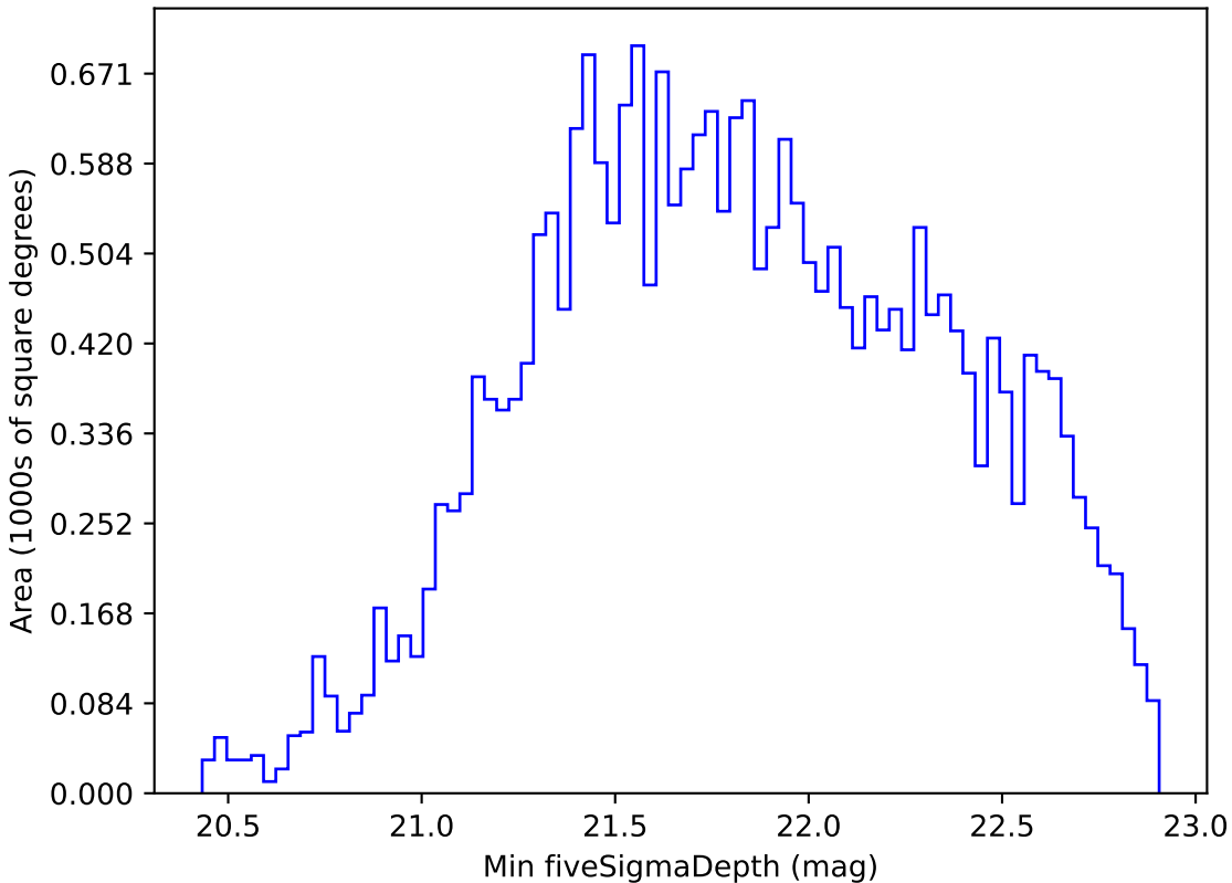
no_high_blob_v3.3_10yrs All sky i band: Min fiveSigmaDepth
