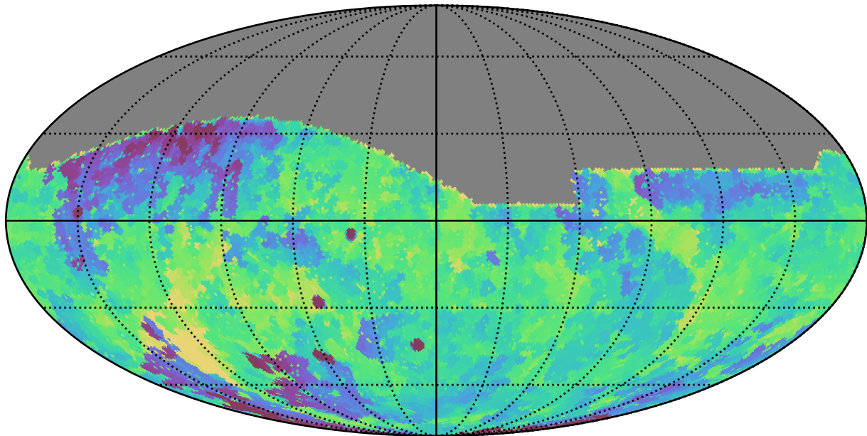
no_high_blob_v3.3_10yrs All sky g band: Min fiveSigmaDepth
