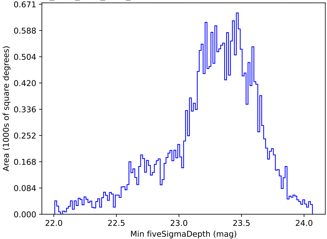
no_high_blob_v3.3_10yrs All sky g band: Min fiveSigmaDepth
