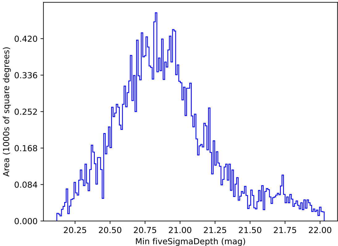
no_high_blob_v3.3_10yrs All sky all bands: Min fiveSigmaDepth
