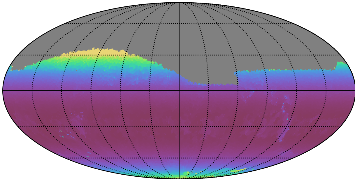
no_high_blob_v3.3_10yrs Yr 1 z band: Min airmass
