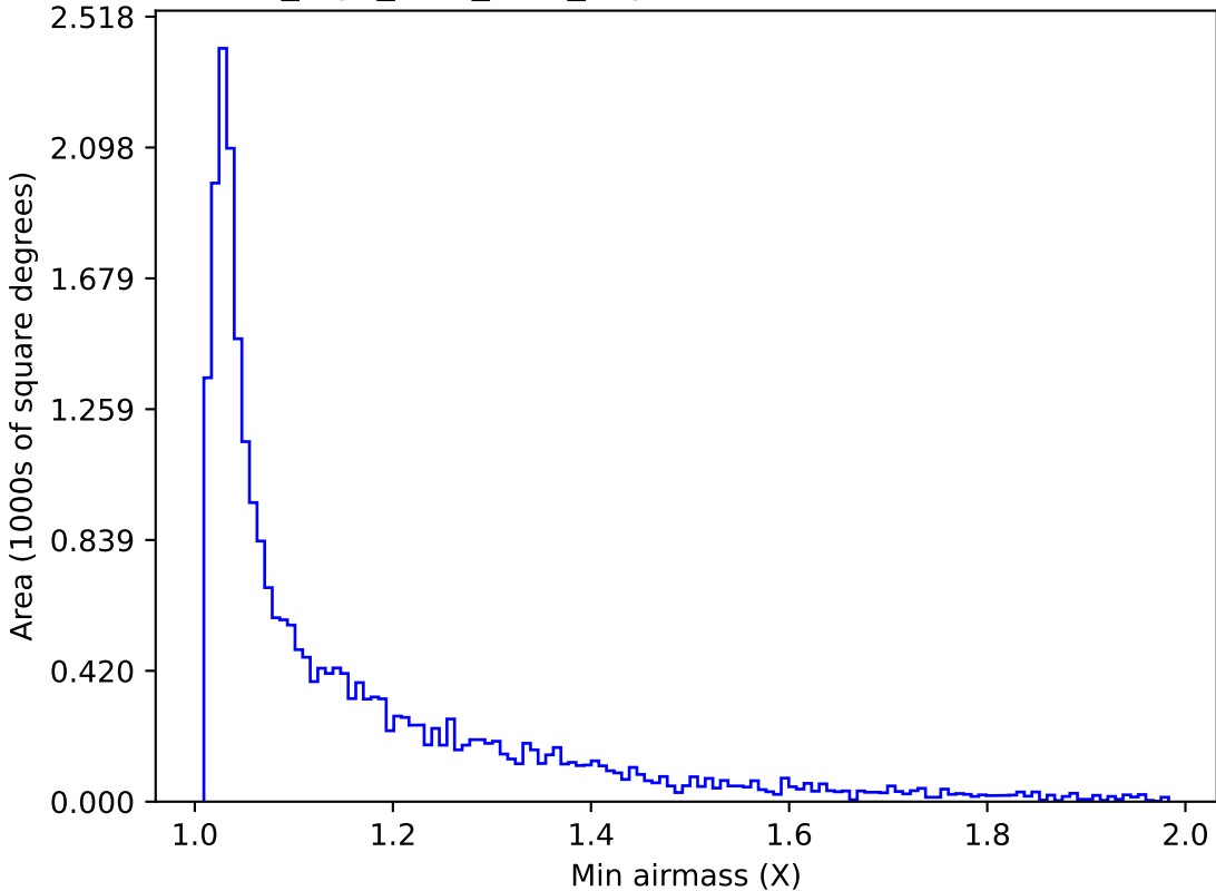
no_high_blob_v3.3_10yrs Yr 1 z band: Min airmass
