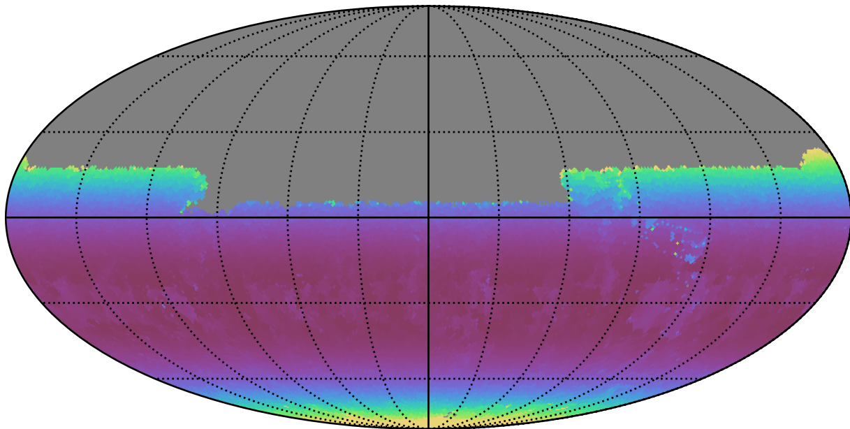
no_high_blob_v3.3_10yrs Yr 1 y band: Min airmass
