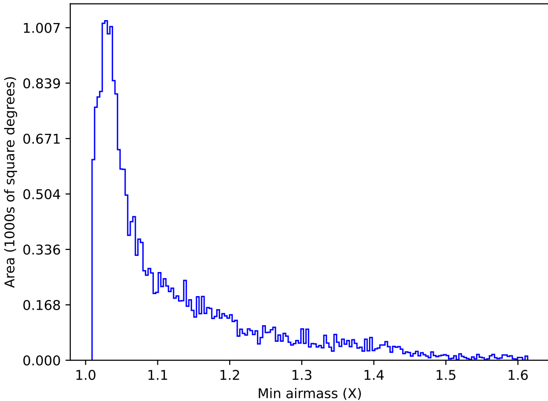
no_high_blob_v3.3_10yrs Yr 1 y band: Min airmass
