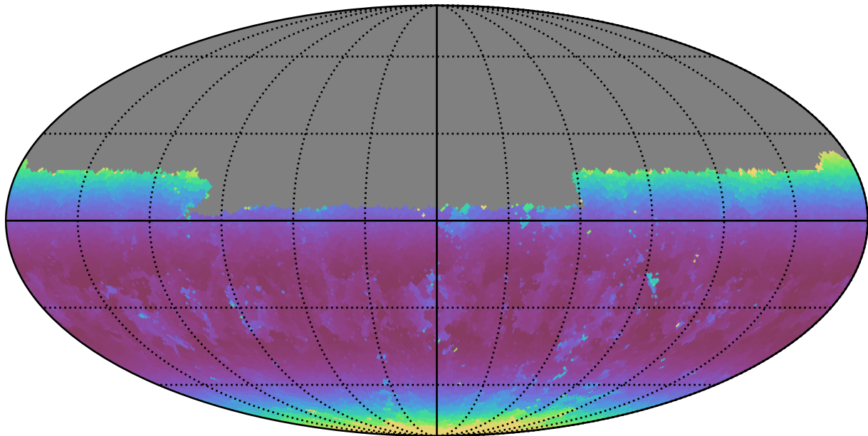
no_high_blob_v3.3_10yrs Yr 1 u band: Min airmass
