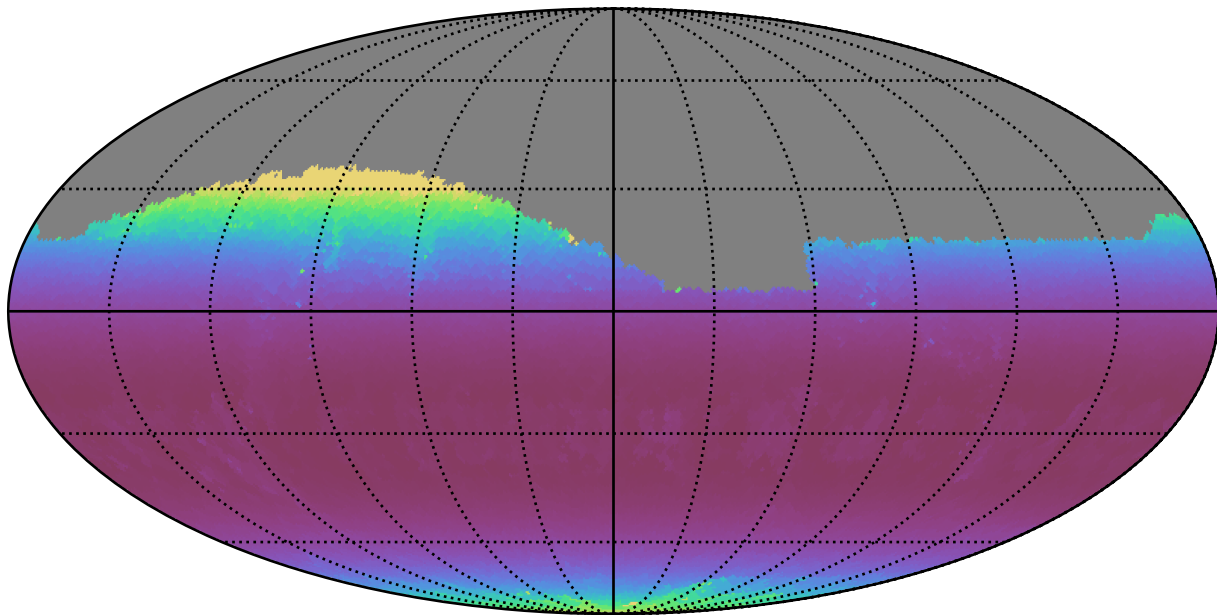
no_high_blob_v3.3_10yrs Yr 1 r band: Min airmass
