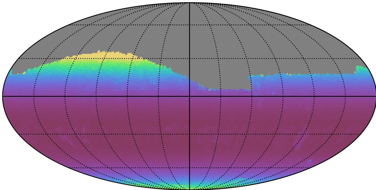
no_high_blob_v3.3_10yrs Yr 1 i band: Min airmass
