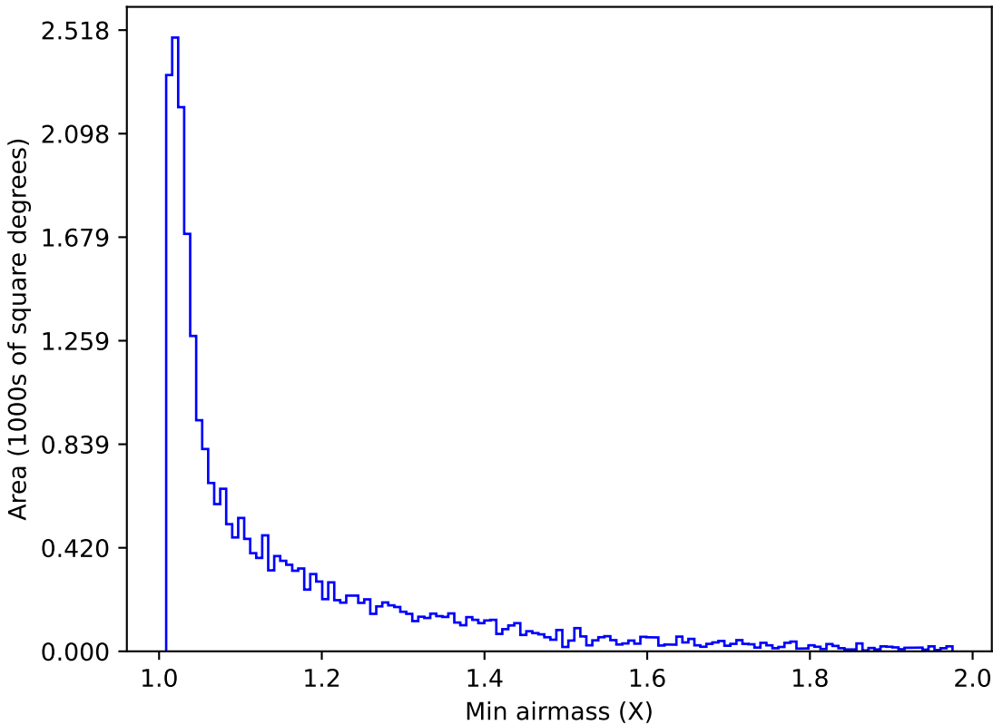
no_high_blob_v3.3_10yrs Yr 1 i band: Min airmass
