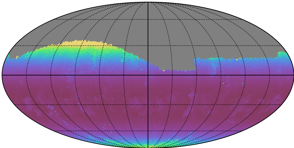
no_high_blob_v3.3_10yrs Yr 1 g band: Min airmass
