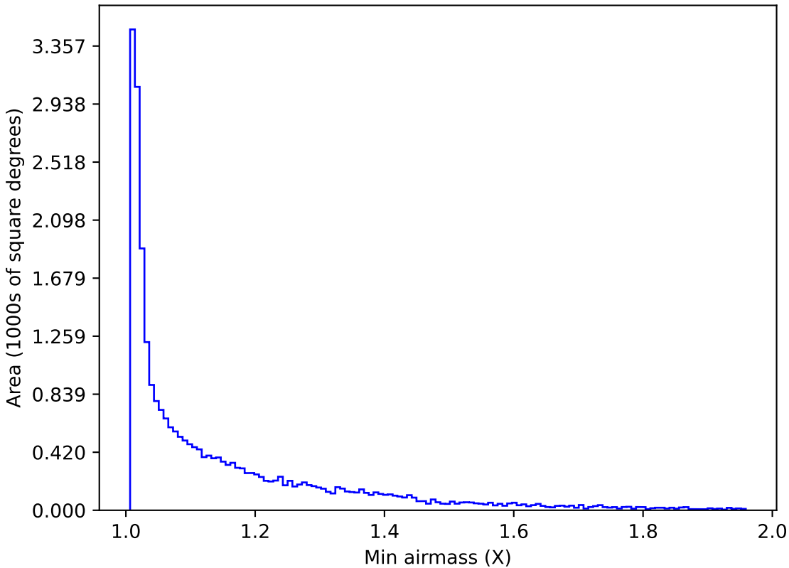
no_high_blob_v3.3_10yrs Yr 1 all bands: Min airmass
