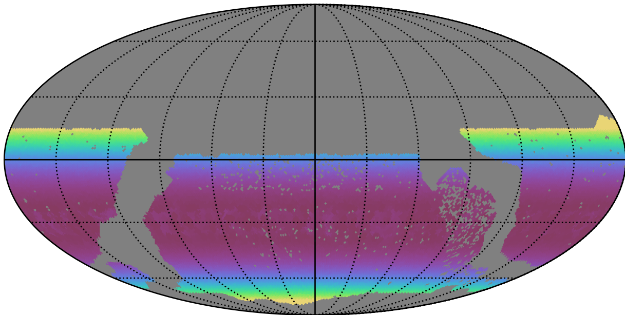
no_high_blob_v3.3_10yrs WFD z band: Min airmass
