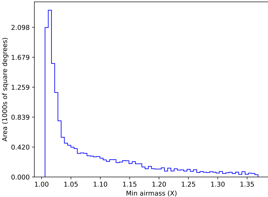
no_high_blob_v3.3_10yrs WFD z band: Min airmass
