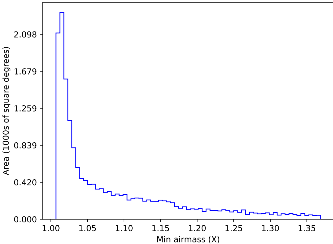
no_high_blob_v3.3_10yrs WFD y band: Min airmass
