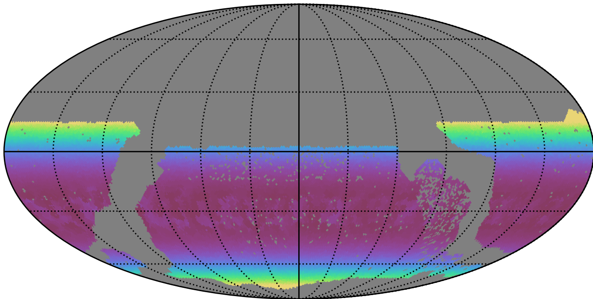
no_high_blob_v3.3_10yrs WFD u band: Min airmass
