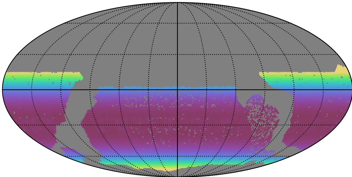
no_high_blob_v3.3_10yrs WFD r band: Min airmass
