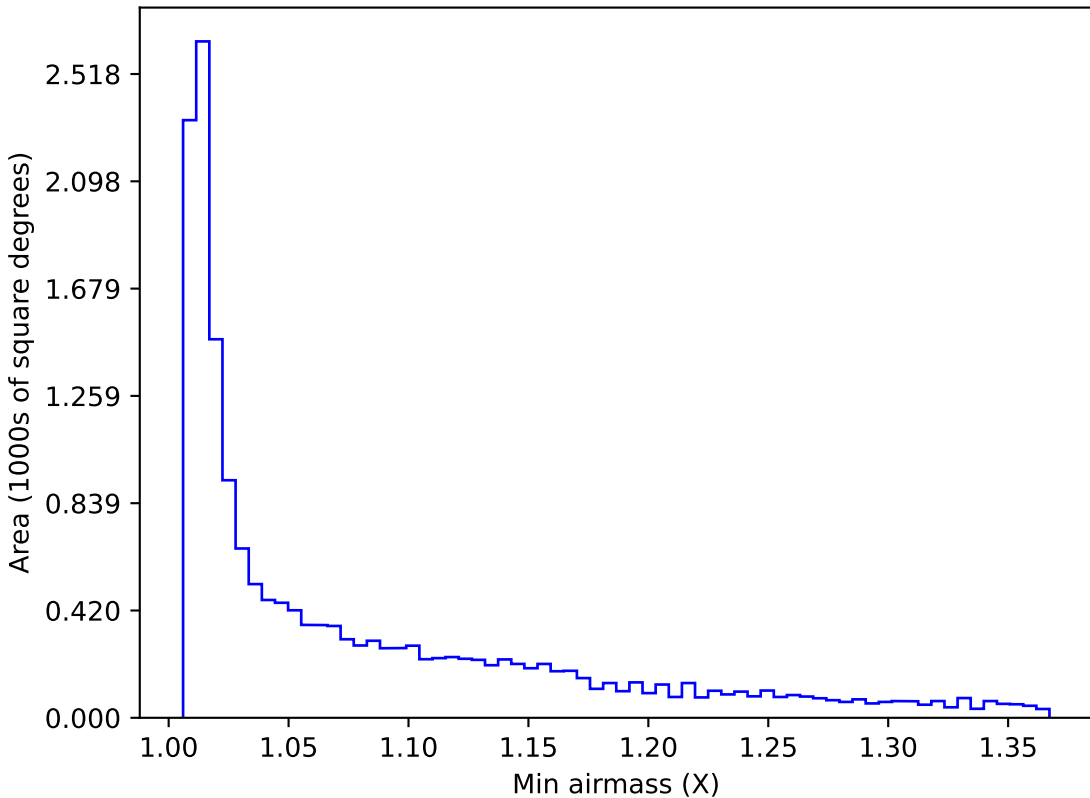
no_high_blob_v3.3_10yrs WFD r band: Min airmass
