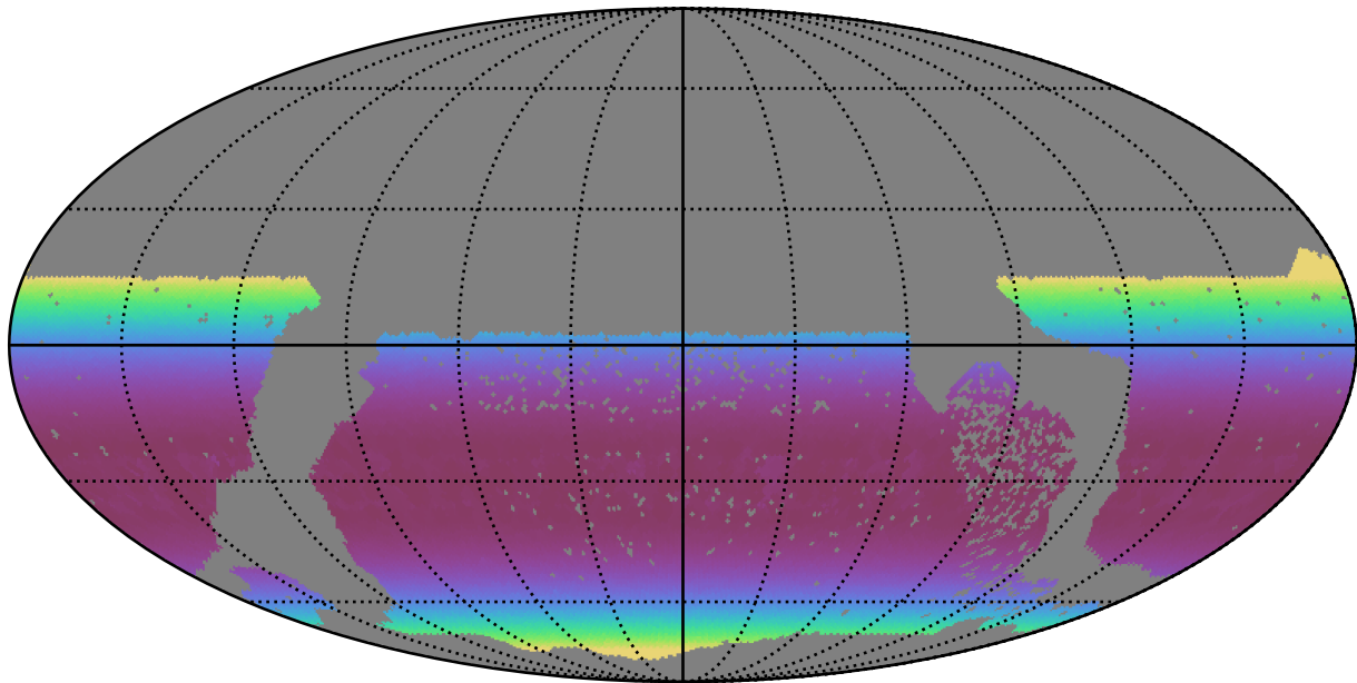
no_high_blob_v3.3_10yrs WFD i band: Min airmass
