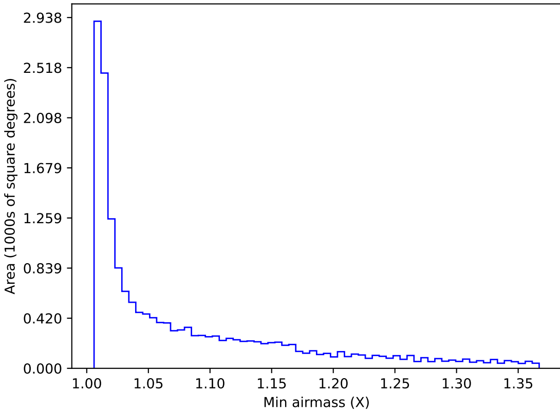
no_high_blob_v3.3_10yrs WFD i band: Min airmass
