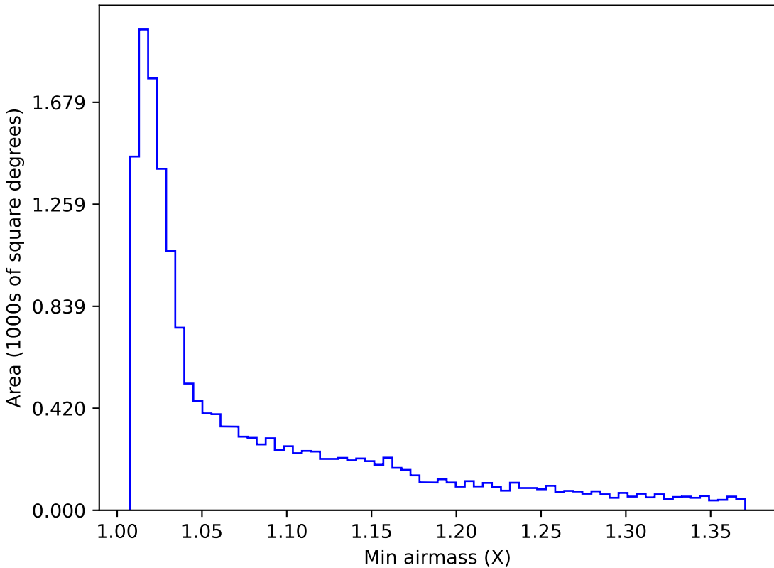
no_high_blob_v3.3_10yrs WFD g band: Min airmass
