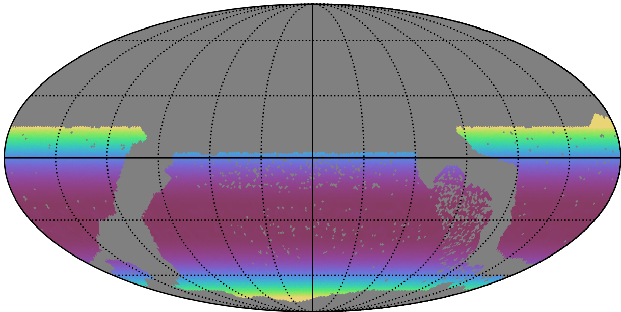
no_high_blob_v3.3_10yrs WFD all bands: Min airmass
