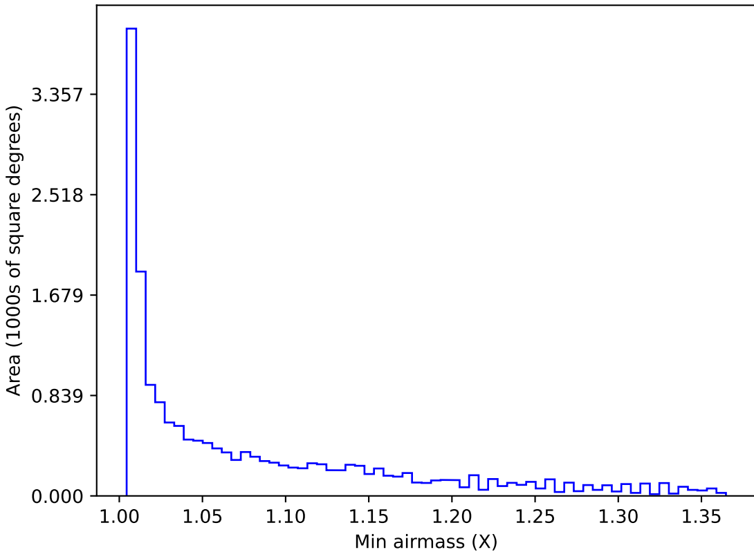
no_high_blob_v3.3_10yrs WFD all bands: Min airmass
