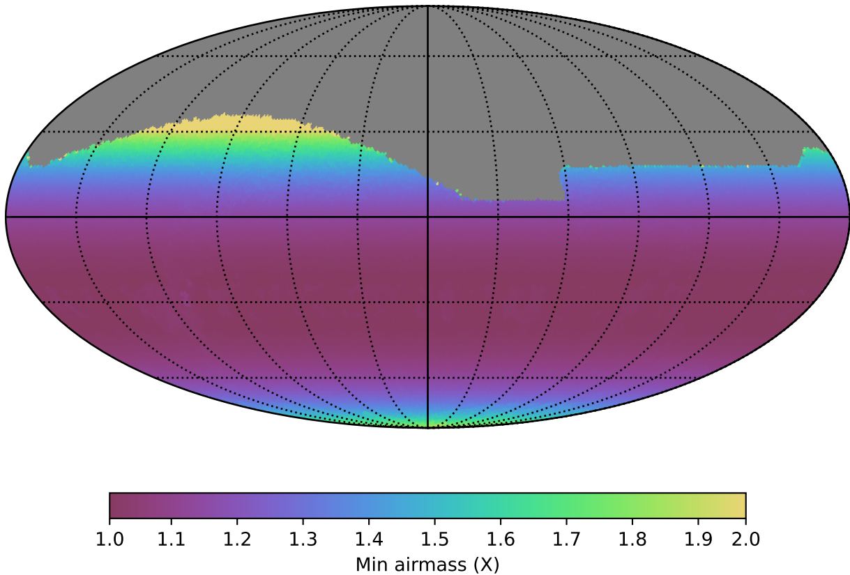
no_high_blob_v3.3_10yrs All sky z band: Min airmass
