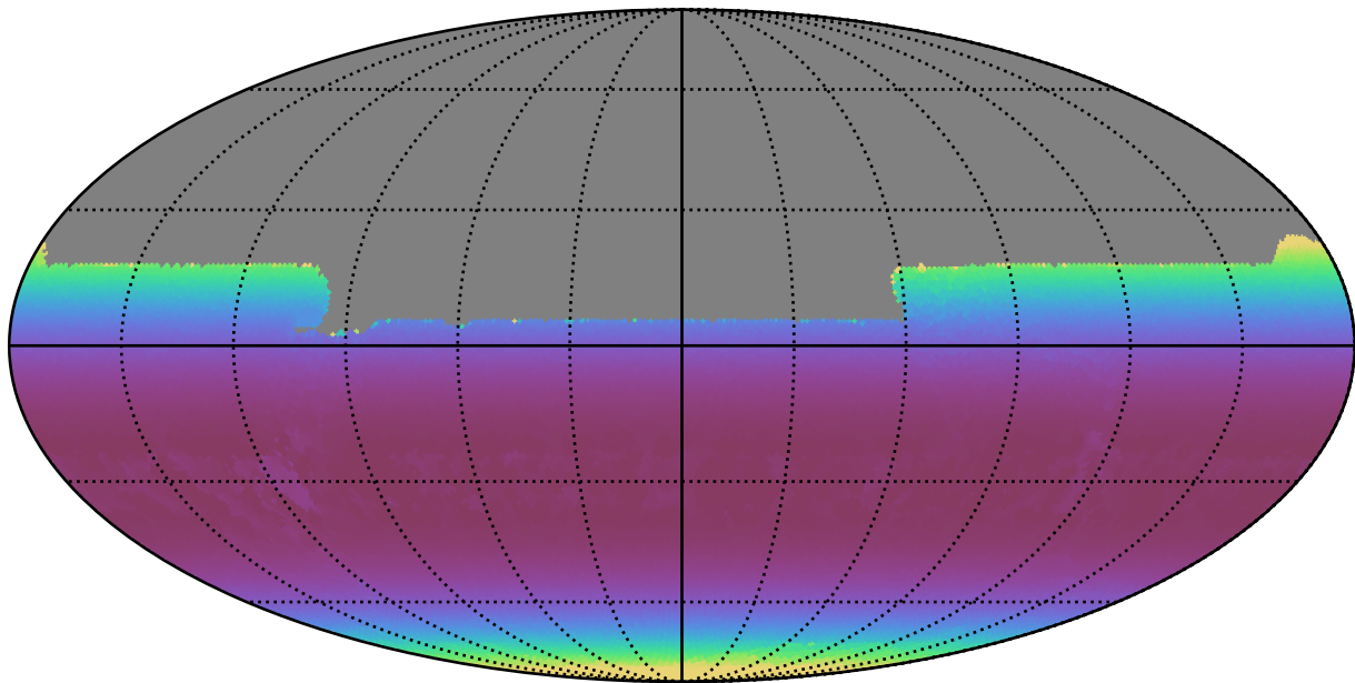
no_high_blob_v3.3_10yrs All sky y band: Min airmass
