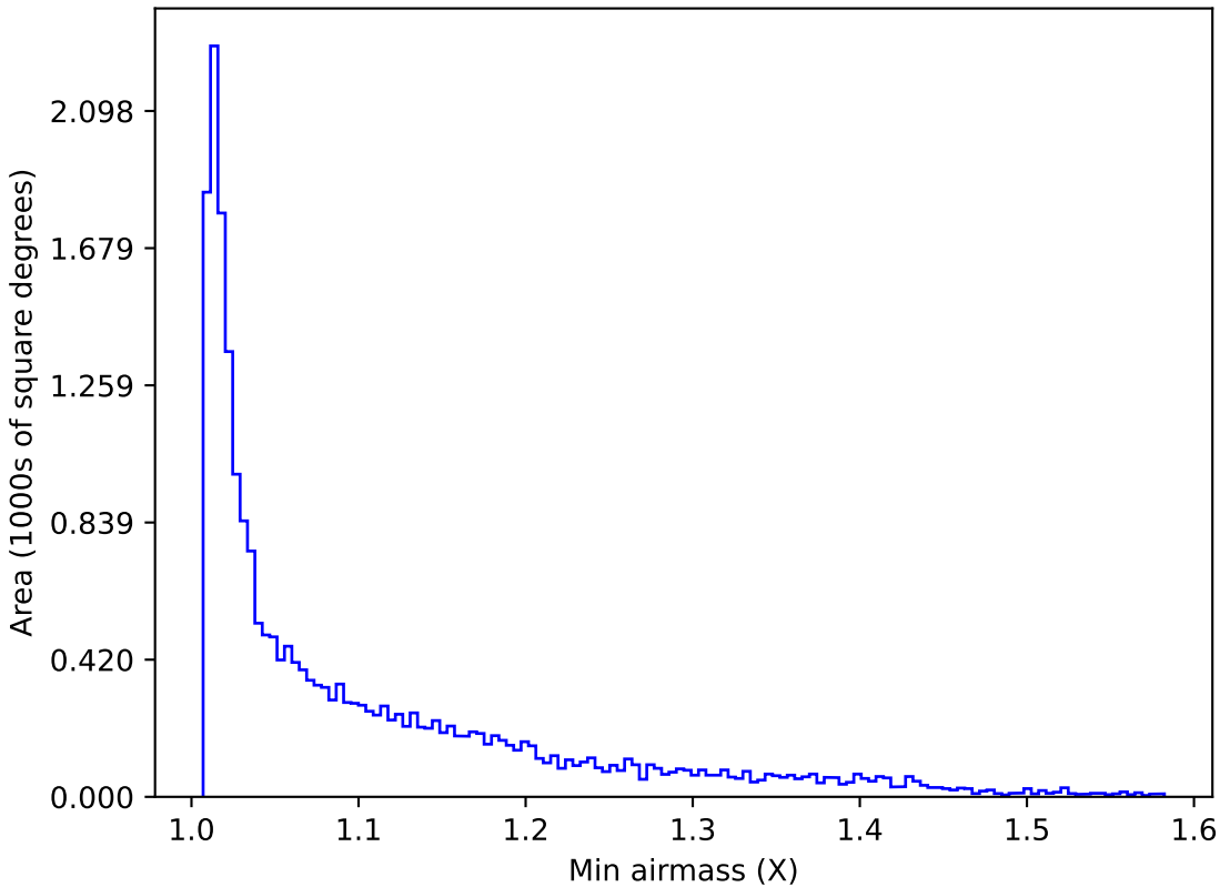
no_high_blob_v3.3_10yrs All sky y band: Min airmass
