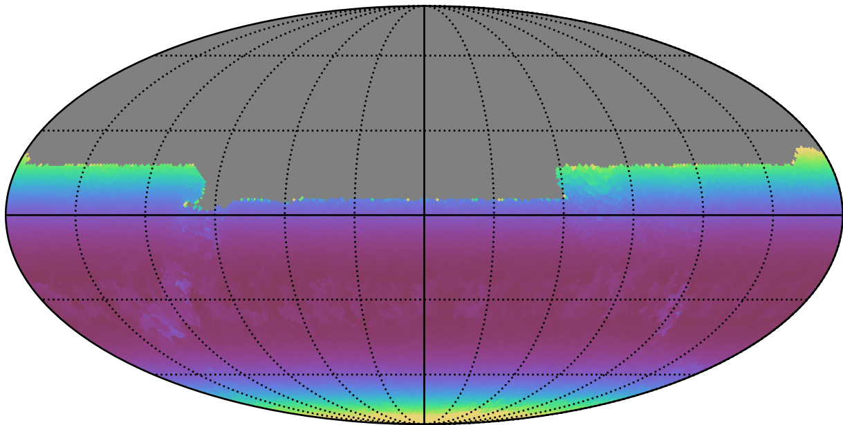
no_high_blob_v3.3_10yrs All sky u band: Min airmass
