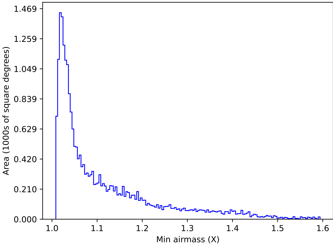
no_high_blob_v3.3_10yrs All sky u band: Min airmass
