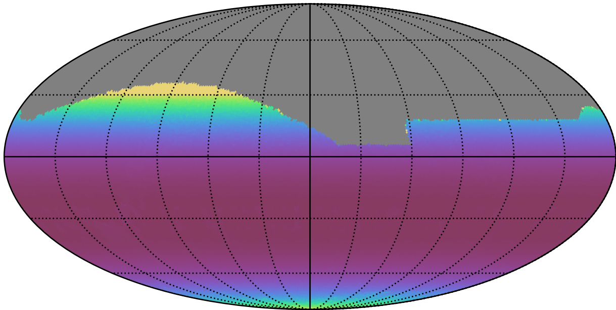
no_high_blob_v3.3_10yrs All sky r band: Min airmass
