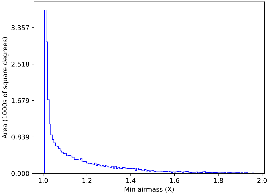
no_high_blob_v3.3_10yrs All sky r band: Min airmass
