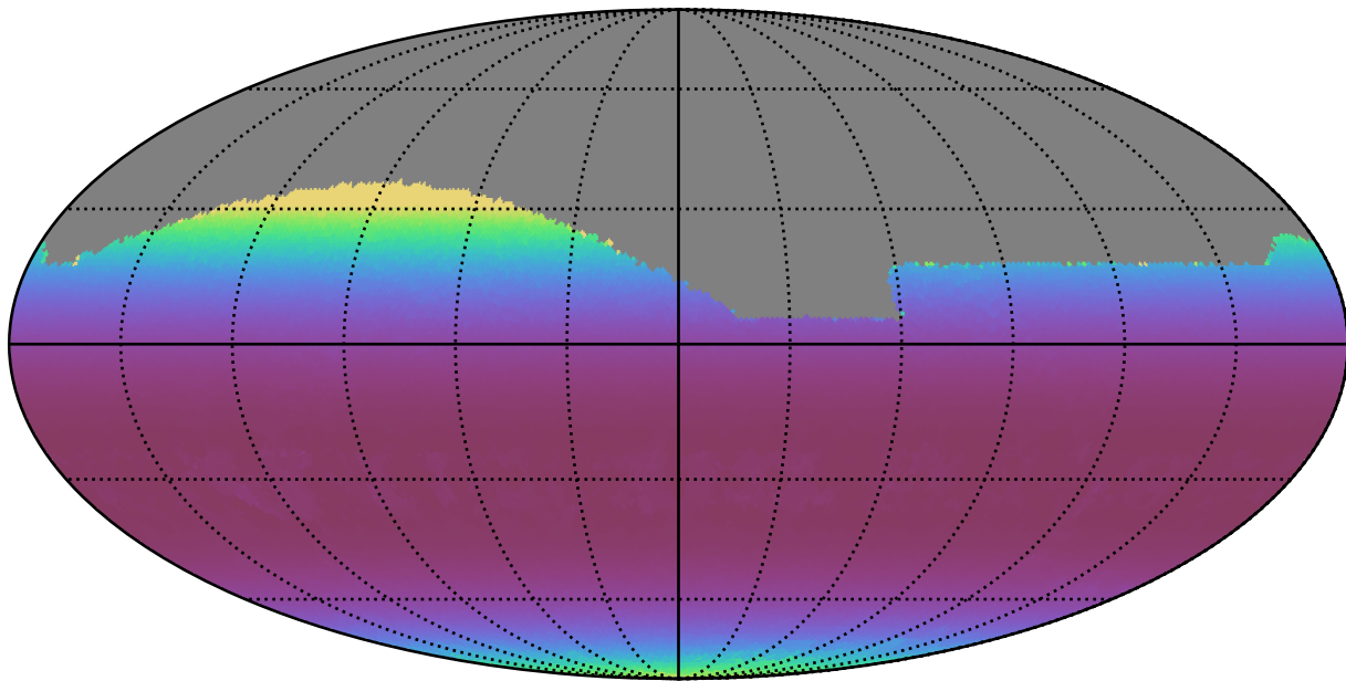
no_high_blob_v3.3_10yrs All sky g band: Min airmass
