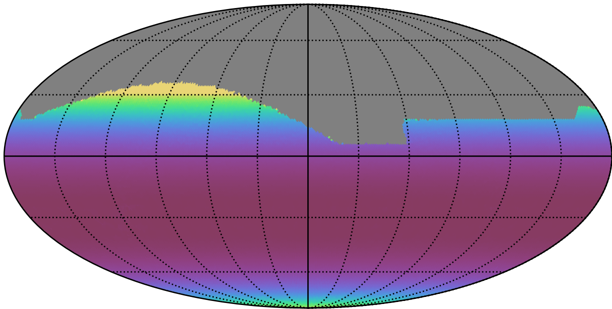
no_high_blob_v3.3_10yrs All sky all bands: Min airmass
