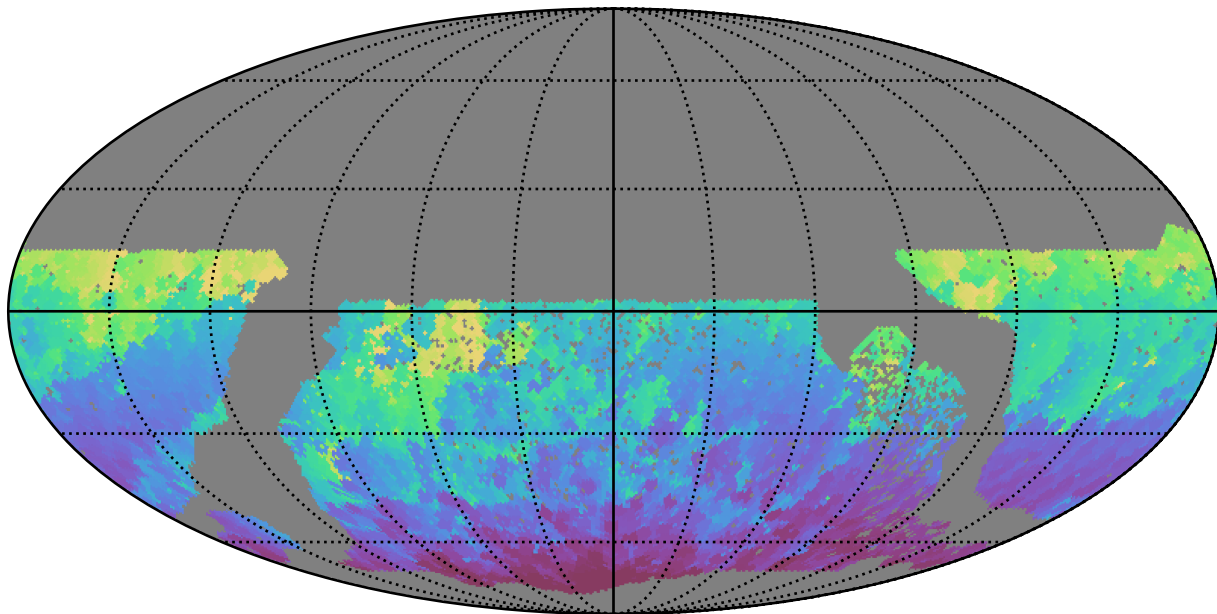
no_high_blob_v3.3_10yrs WFD z band: Min HA
