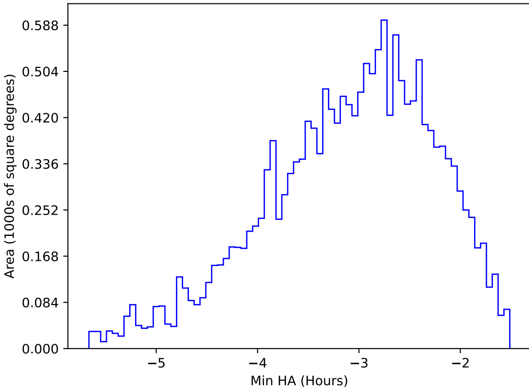
no_high_blob_v3.3_10yrs WFD u band: Min HA
