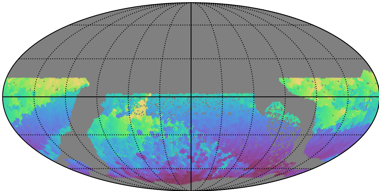
no_high_blob_v3.3_10yrs WFD r band: Min HA
