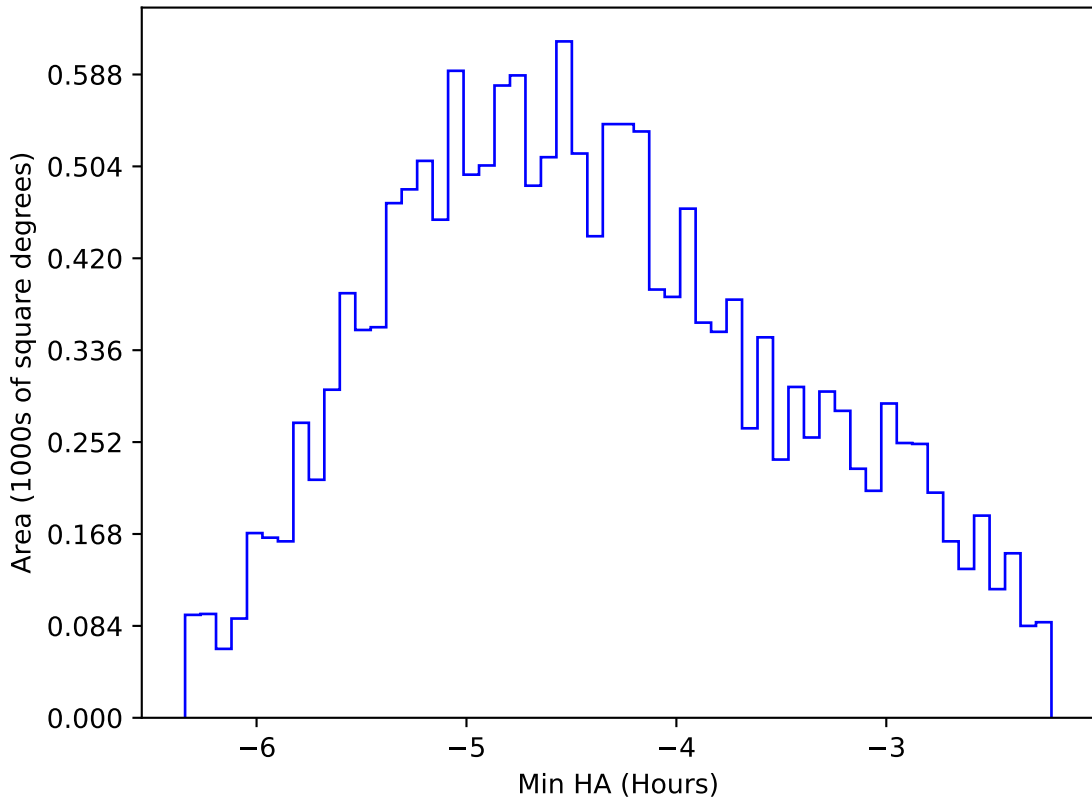
no_high_blob_v3.3_10yrs WFD r band: Min HA
