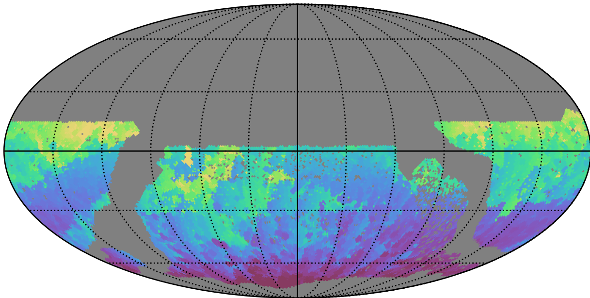
no_high_blob_v3.3_10yrs WFD i band: Min HA
