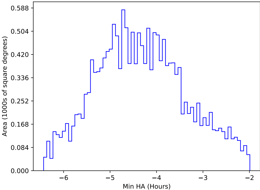
no_high_blob_v3.3_10yrs WFD i band: Min HA
