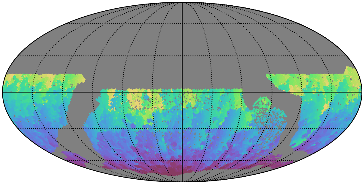
no_high_blob_v3.3_10yrs WFD g band: Min HA
