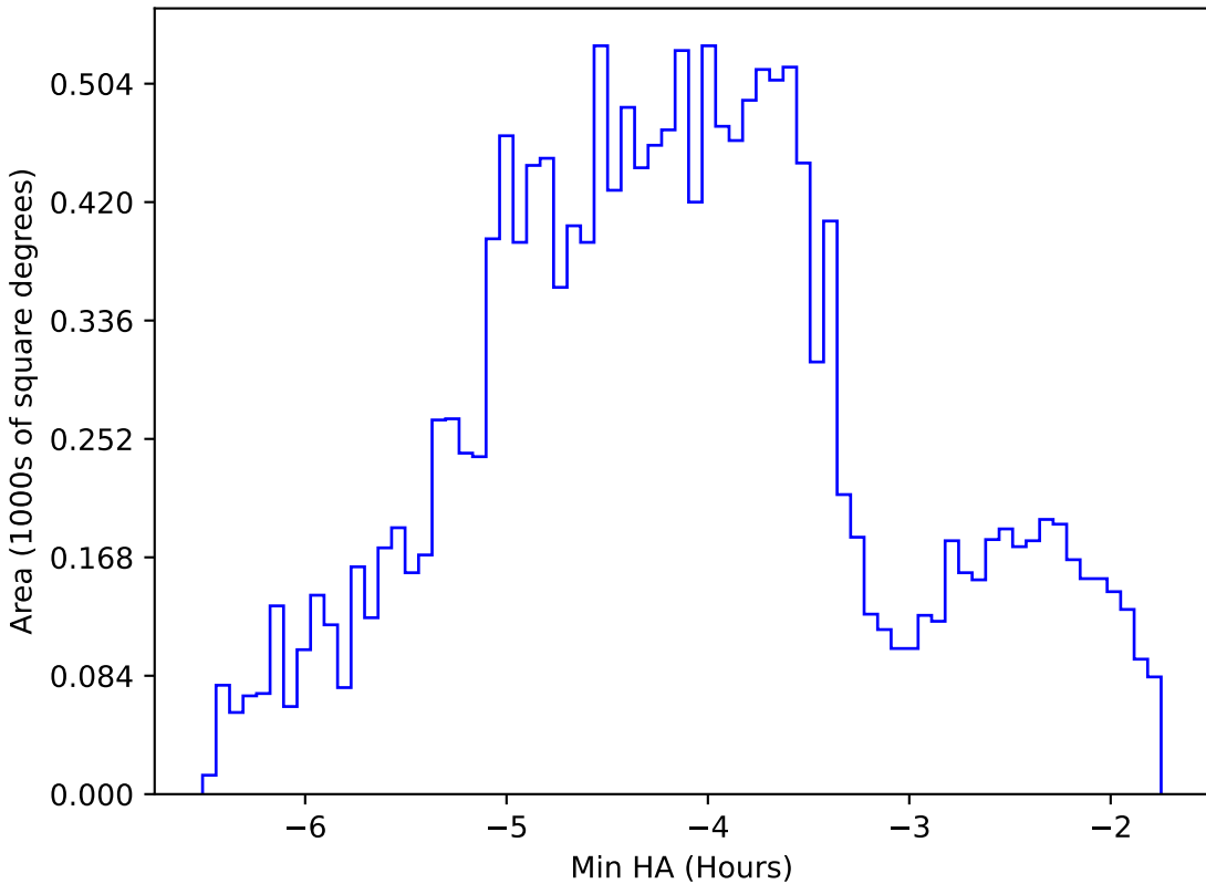
no_high_blob_v3.3_10yrs WFD g band: Min HA
