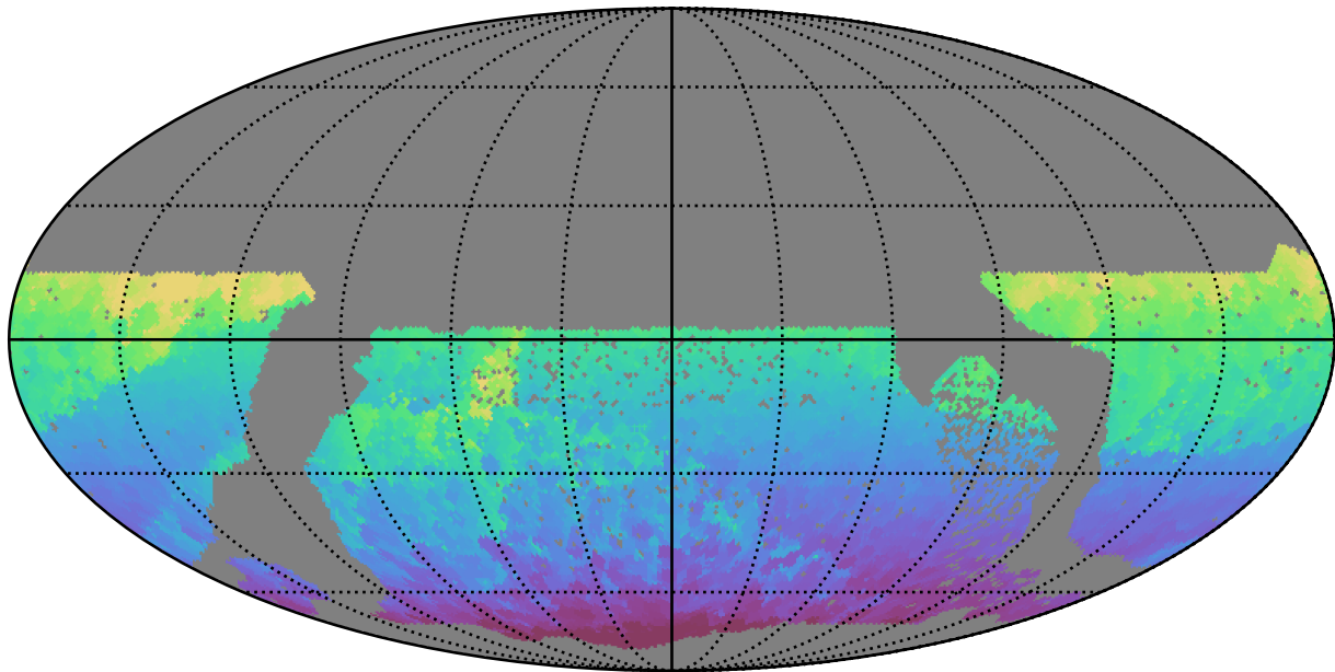
no_high_blob_v3.3_10yrs WFD all bands: Min HA
