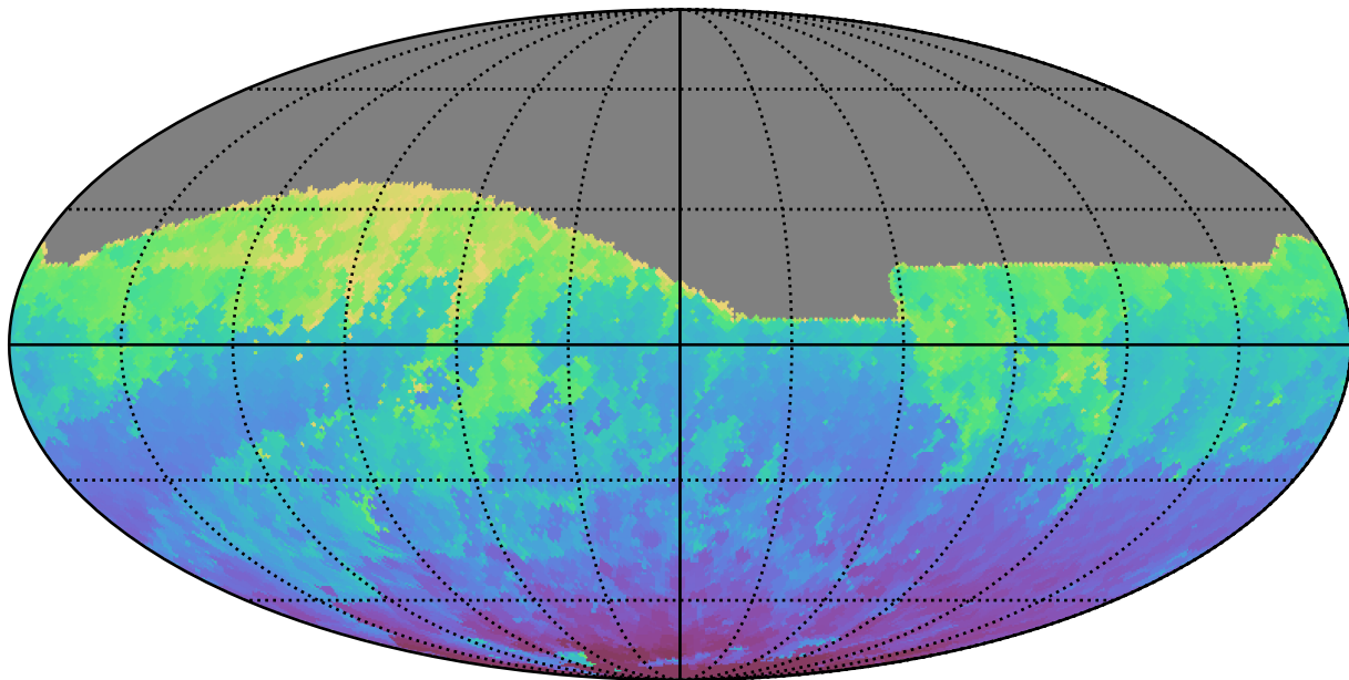
no_high_blob_v3.3_10yrs All sky z band: Min HA
